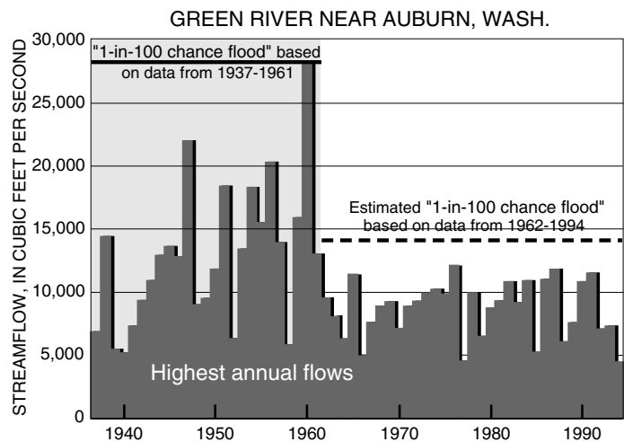
The completion of Howard Hanson Dam on the Green River has decreased the magnitude of the "1-in-100 chance flood" at Auburn, Wash. since 1961.
