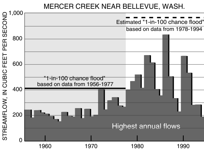
Rapid urban development in the Mercer Creek Basin since 1977 has increased the estimated magnitude of the "1-in-100 chance flood" at Bellevue, Wash.
